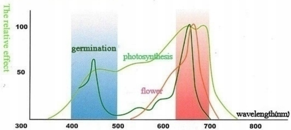
LED wavelength relative effect chart
